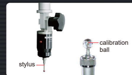
probe (optional) includes Ø1mm and Ø2mm styli, Ø20mm calibration ball, measuring accuracy is 5μm
